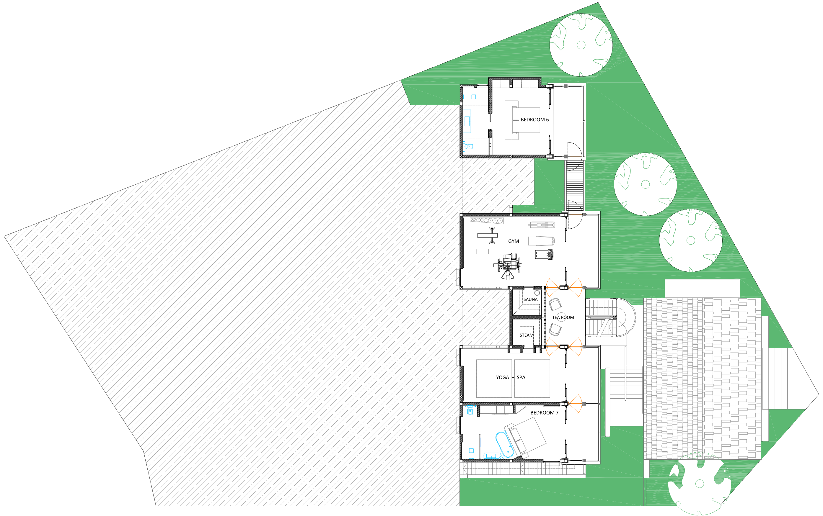
FITNESS + BEDROOMS FLOOR LEVEL SAMSARA VILLA 10
